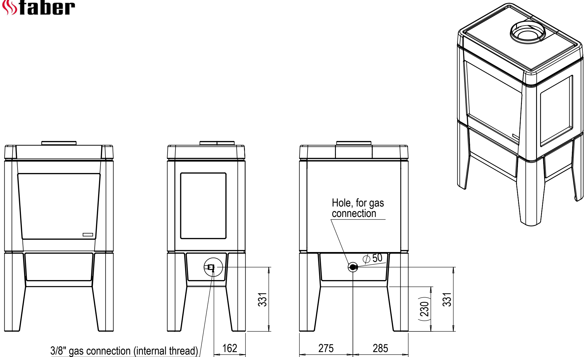
Dimensional drawing position gas connection Odense
