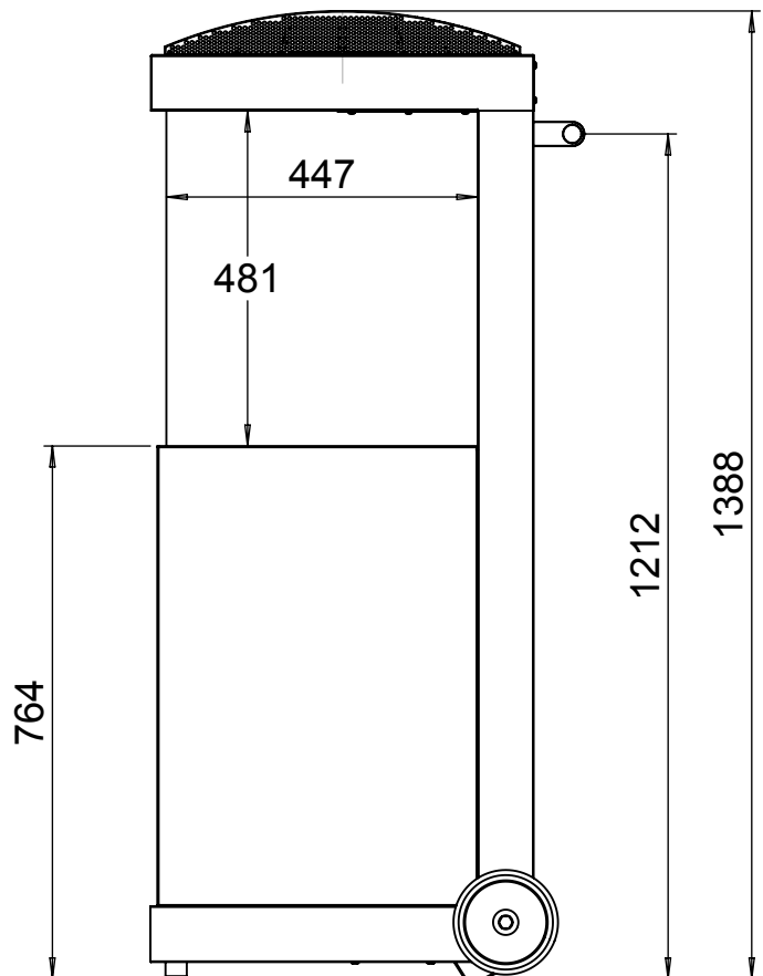
Dimensional drawing The Buzz
