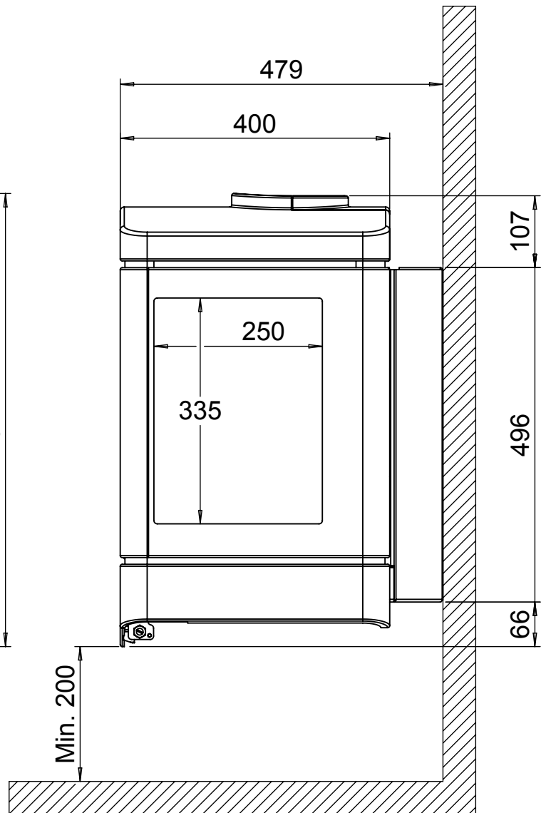
Dimensional drawing Skive
