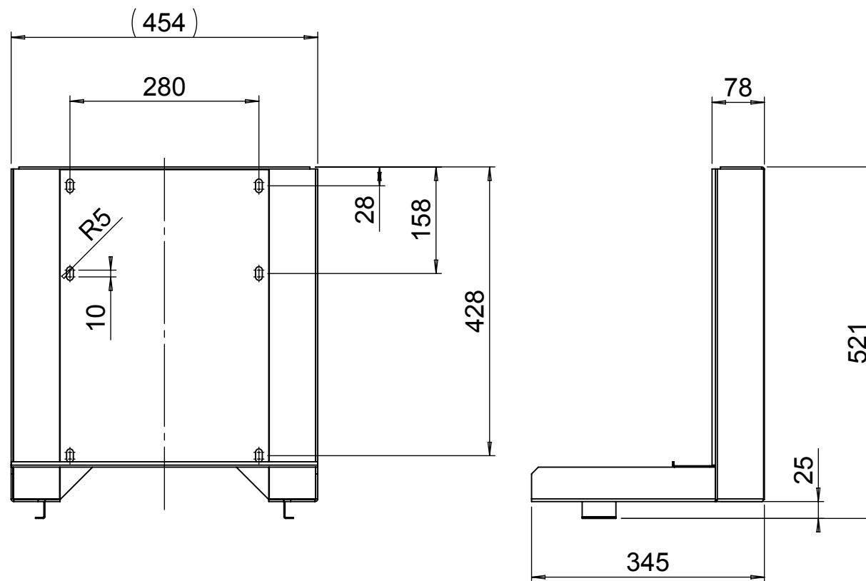
Dimensional drawing wall bracket Skive
