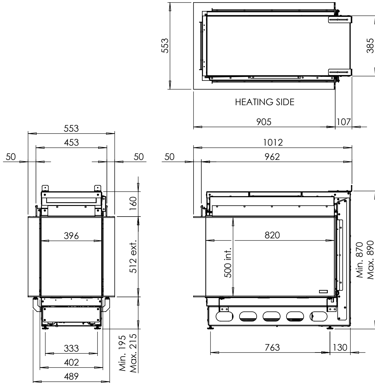
Dimensional Drawing e-Matrix heat 800x500 RD (MkII)
